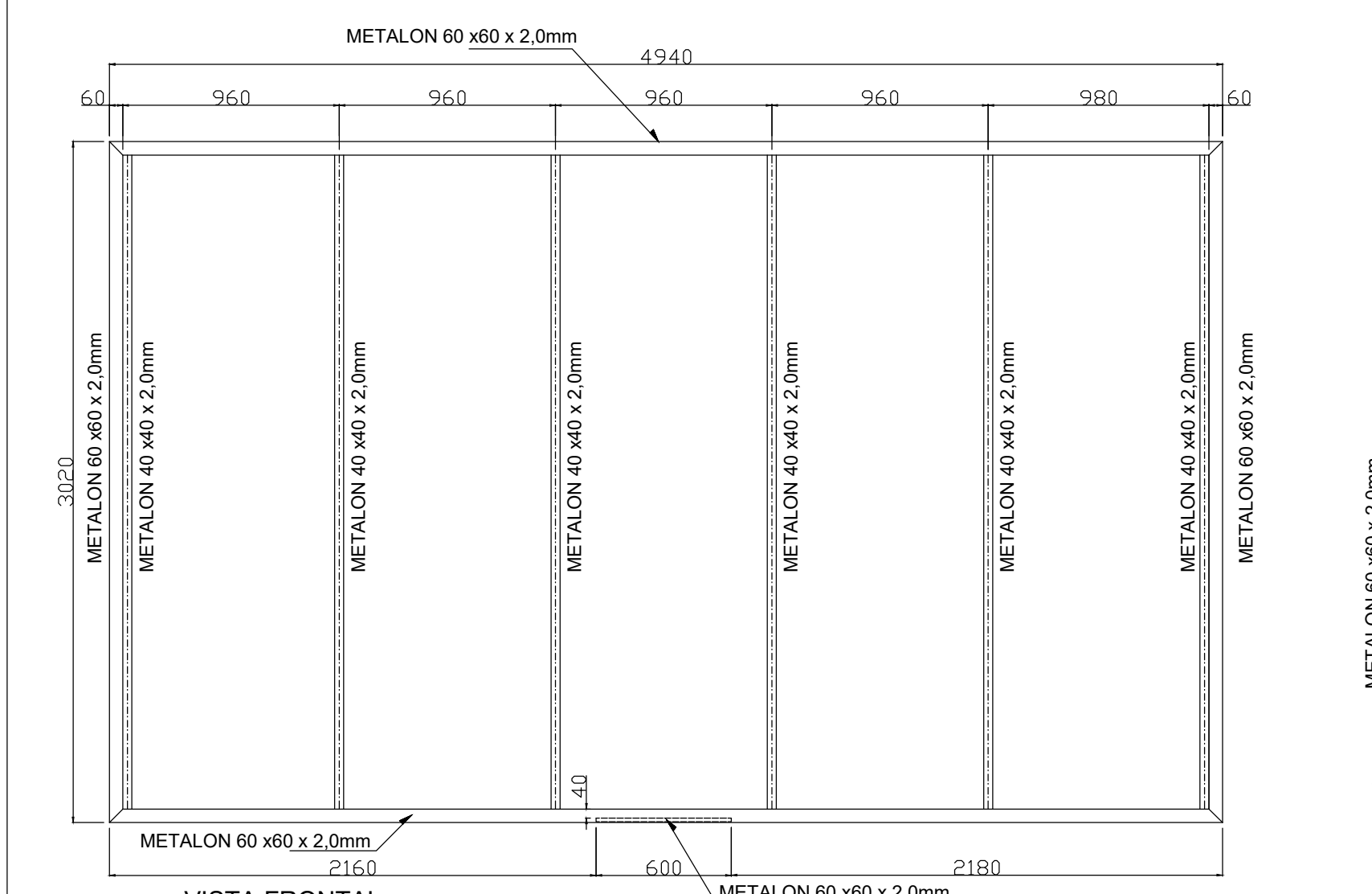
VISTA FRONTAL
